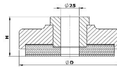
Bolt-through 25mm diameter bore
