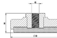
Adapter with M20x2.5 Inner Thread and M40x2 External Thread
